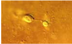
Figure 3: Flagellates have one or two flagella which they use to propel or pull their way through soil. A flagellum can be seen extending from the protozoan on the left. The tiny specks are bacteria.
