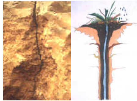
Figure 4: Some worms live in permanent vertical burrows such as these. Others move horizontally near the surface, filling their burrow with casts as they move.
