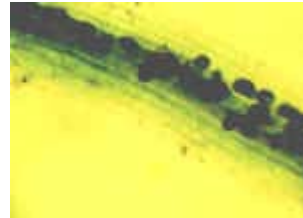
Figure 4: The dark, round masses inside the cells of this clover root are vesicles for the arbuscular mycorrhizal fungus (AM).
